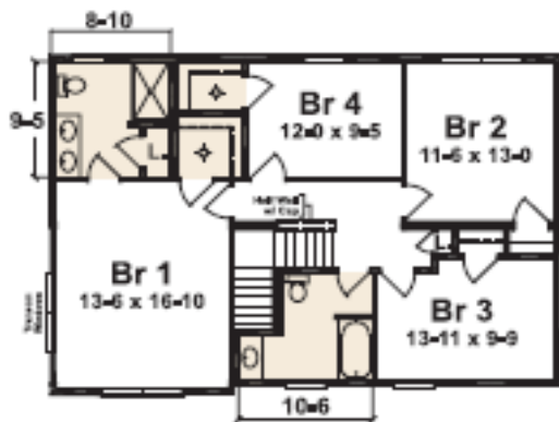
BRAXTON III 2ND FLOOR PLAN
