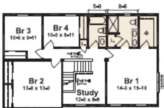
BROCKTON III 2ND FLOOR PLAN
