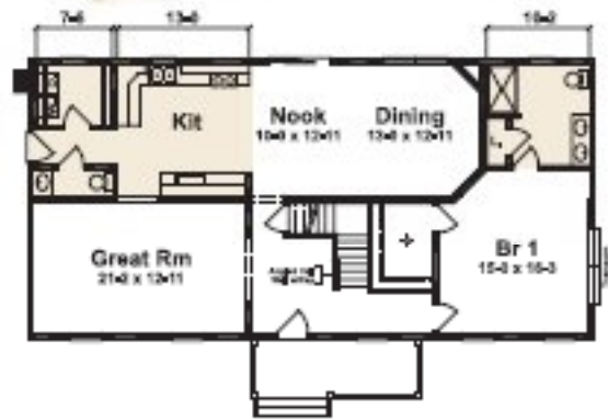
BRIGHTON II 1ST FLOOR PLAN 27-6 x 56-0 2918 Sq. Ft.
