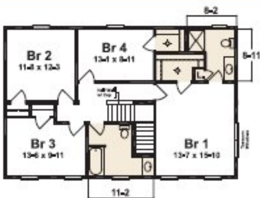
BRAXTON I 2ND FLOOR PLAN
