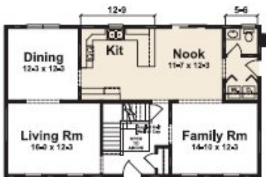
BROCKTON I 1ST FLOOR PLAN 26-0 X 44-0 2288 Sq. Ft.
