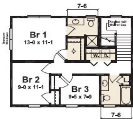
BELMONT I 2ND FLOOR PLAN
