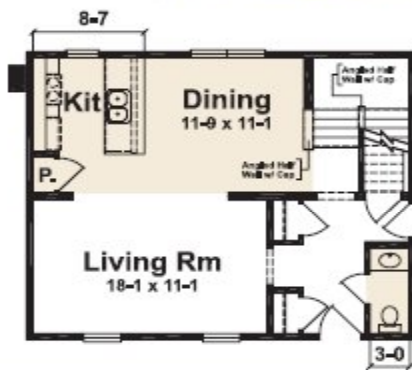
BELMONT I 1ST FLOOR PLAN 23-8 X 30-0 1420 Sq. Ft.
