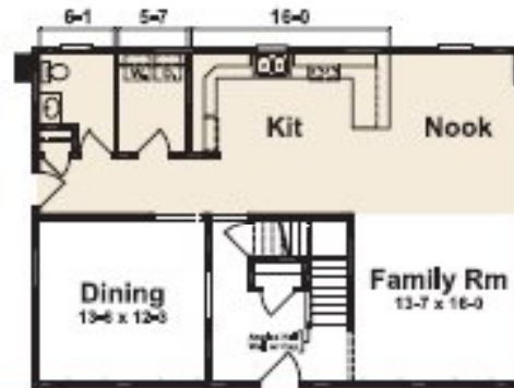
BRAXTON II 1ST FLOOR PLAN 27-6 X 40-0 2200 Sq. Ft.
