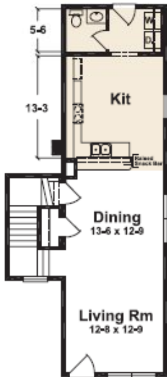
BAXTER I 1ST FLOOR PLAN 21-0 X 48-0 1520 Sq. Ft.
