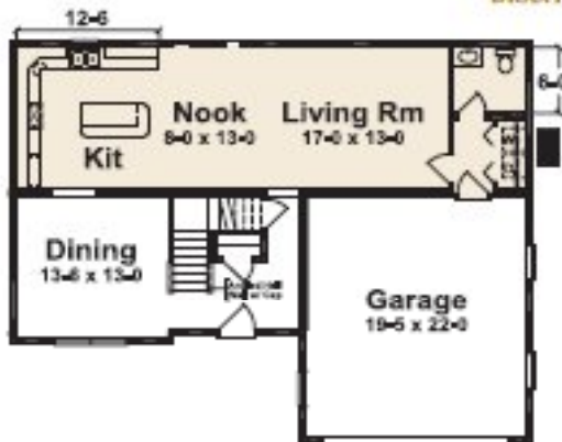
BRAXTON III 1ST FLOOR PLAN 26-9/27-6/36-6 X 46-1/40 2092 Sq. Ft.
