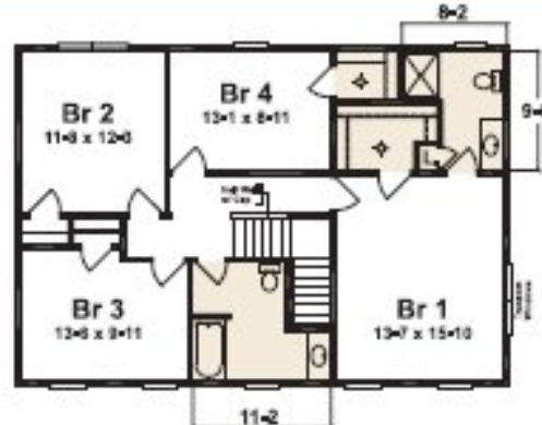
BRAXTON II 2ND FLOOR PLAN
