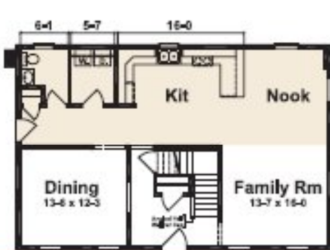
BRAXTON I 1ST FLOOR PLAN 26-0 X 40-0 2080 Sq. Ft.
