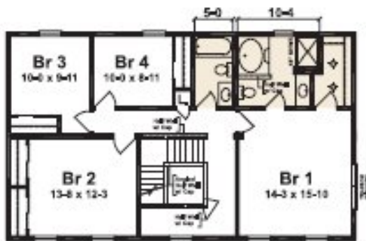
BROCKTON I 2ND FLOOR PLAN
