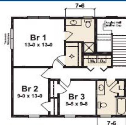
BELMONT III 2ND FLOOR PLAN
