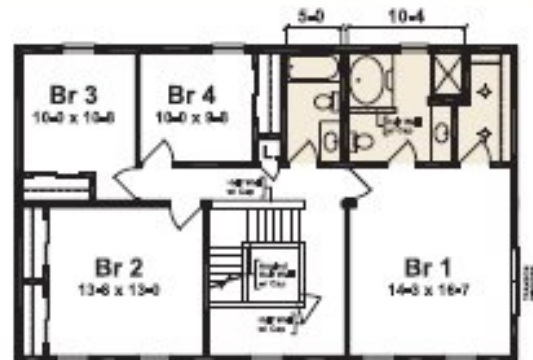
BROCKTON II 2ND FLOOR PLAN
